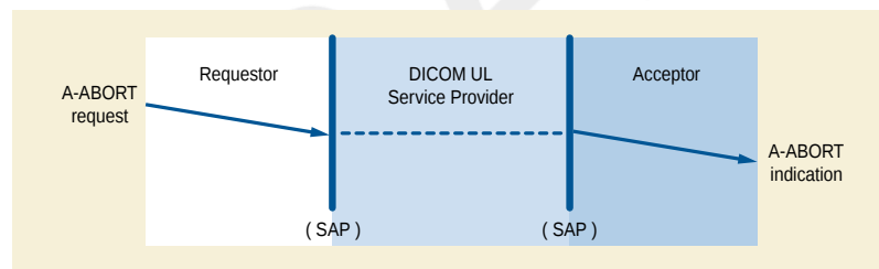
Figure 7-3. Association User Initiated Abort
