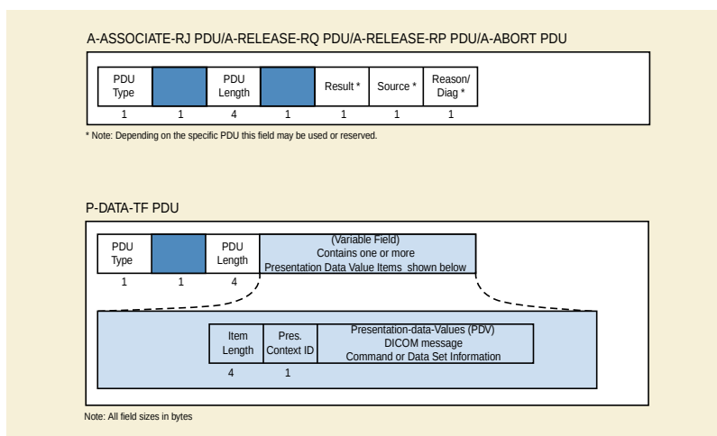
Figure 9-2. Protocol Data Units Structure and Encoding
